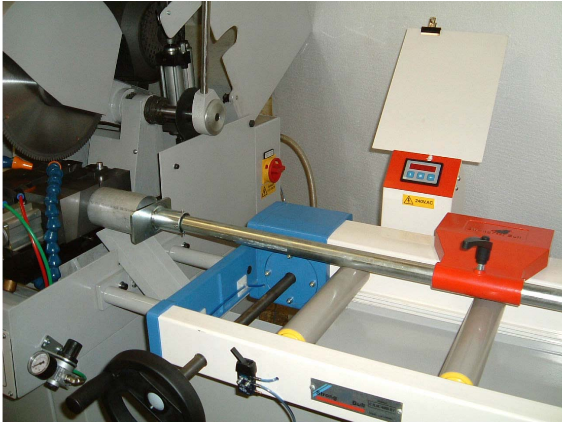
Adjustable height Outfeed roller table fitted to a cutting machine. End stop has been extended and end stop positioning handle is visible
