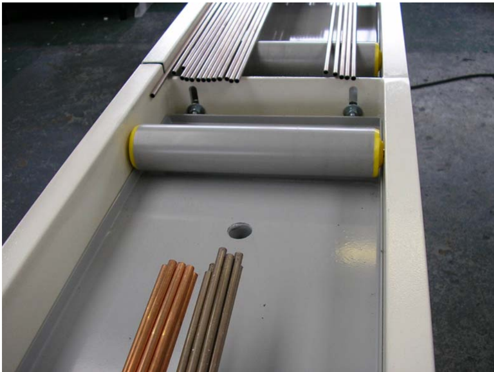
Infeed roller table with drip tray and drain fitted to prevent coolant running away down the tubes
